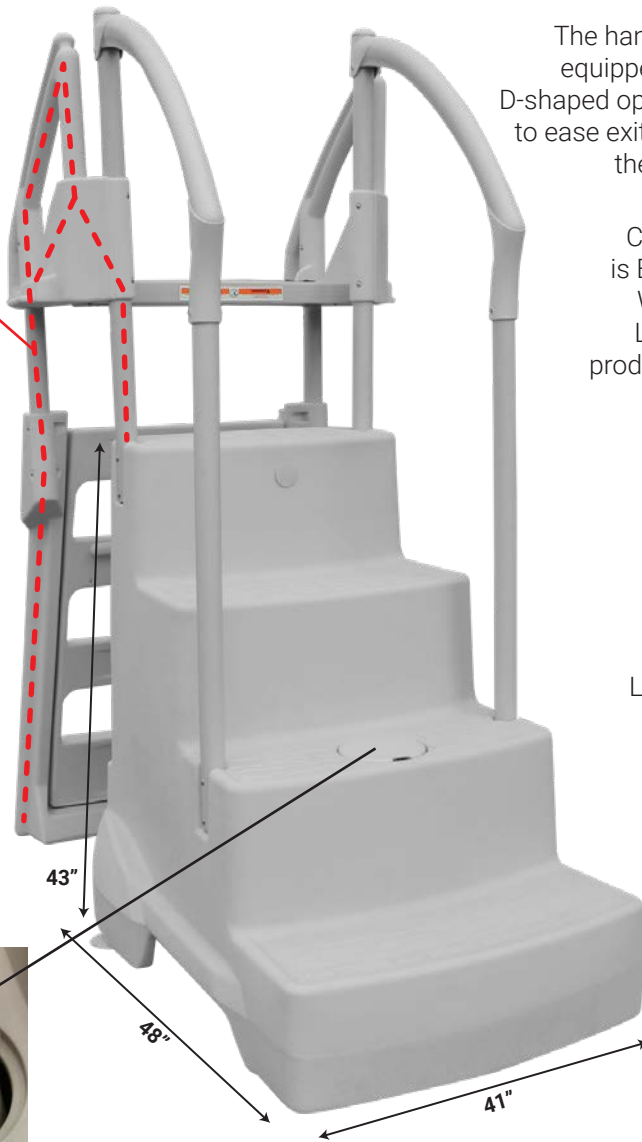
Massive grab-rail
